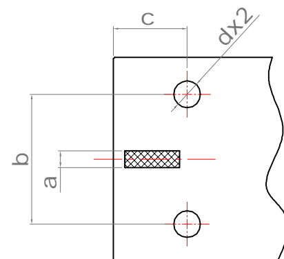
Recommended PCB Soldering Pattern
